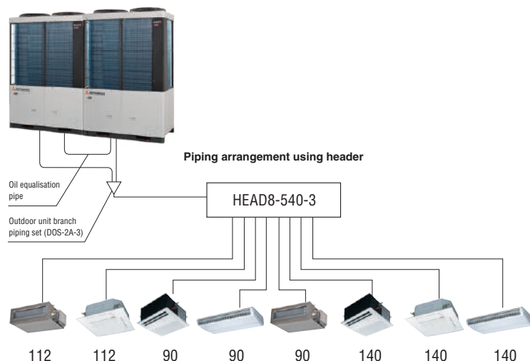
Outdoor unit side branching pipe set
