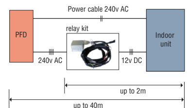
PFD4-15WR-E (option)
