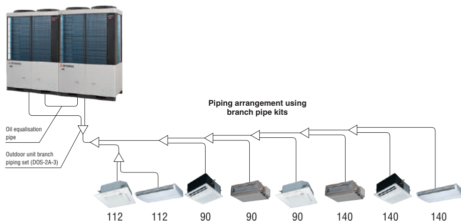
Outdoor unit side branching pipe set
